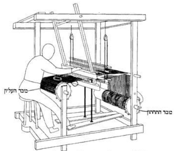
Weaving machine
